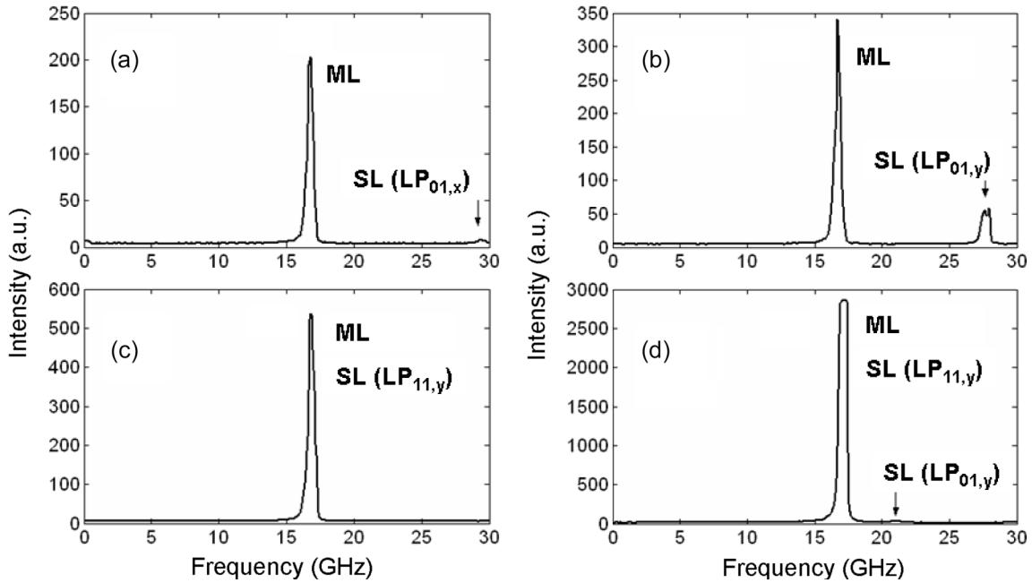
Fig. 9. Polarization mode competition when the detuning is fixed at 100 GHz. (a) VCSEL emits in horizontal before PS, P_{inj} = 3.26 mW. (b) After PS to vertical polarization, P_{inj} = 5.24 mW. (c) Injection locking of the LP_{11,y} mode, P_{inj} = 7.99 mW. (d) Injection locking of the LP_{11,y} mode with relatively weak recovery of the VCSEL fundamental mode P_{inj} = 18 mW.
