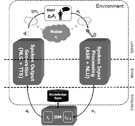
Fig. 1. Spoken Dialogue Model
