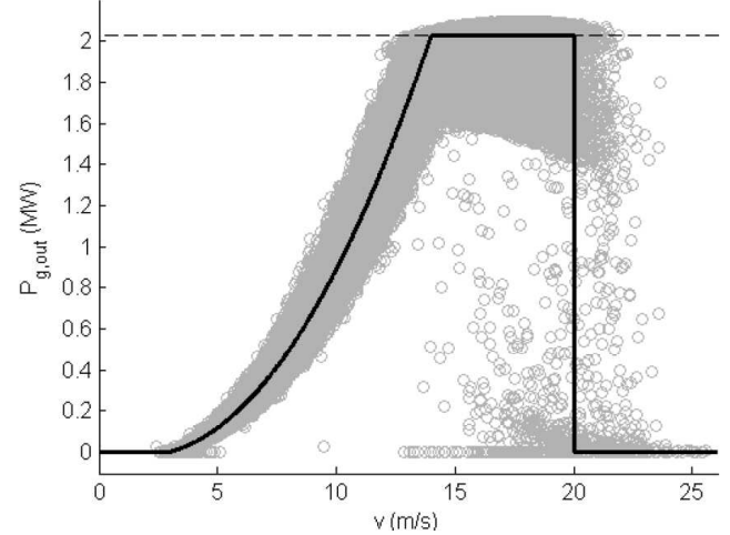
Figure 6: Joint probability function (grey) for a wind time series of 10.00 m/s annual mean. The steady-state power curve is represented in black.
