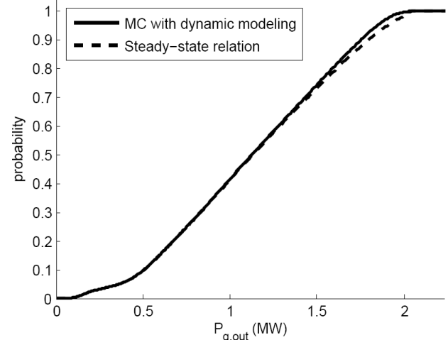
Figure 10: Cumulative distribution function of a 10 turbine wind farm generation obtained with dynamic modeling and steady-state power curve with an annual mean wind speed of 10 m/s.
