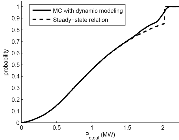
Figure 8: Cumulative distribution function of the wind turbine generation obtained with dynamic modeling and steady-state power curve with an annual mean wind speed of 10.00 m/s.
