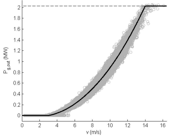
Figure 5: Joint probability function (grey) for a wind time-series of 5.46 m/s annual mean. The steady-state power curve is represented in black.
