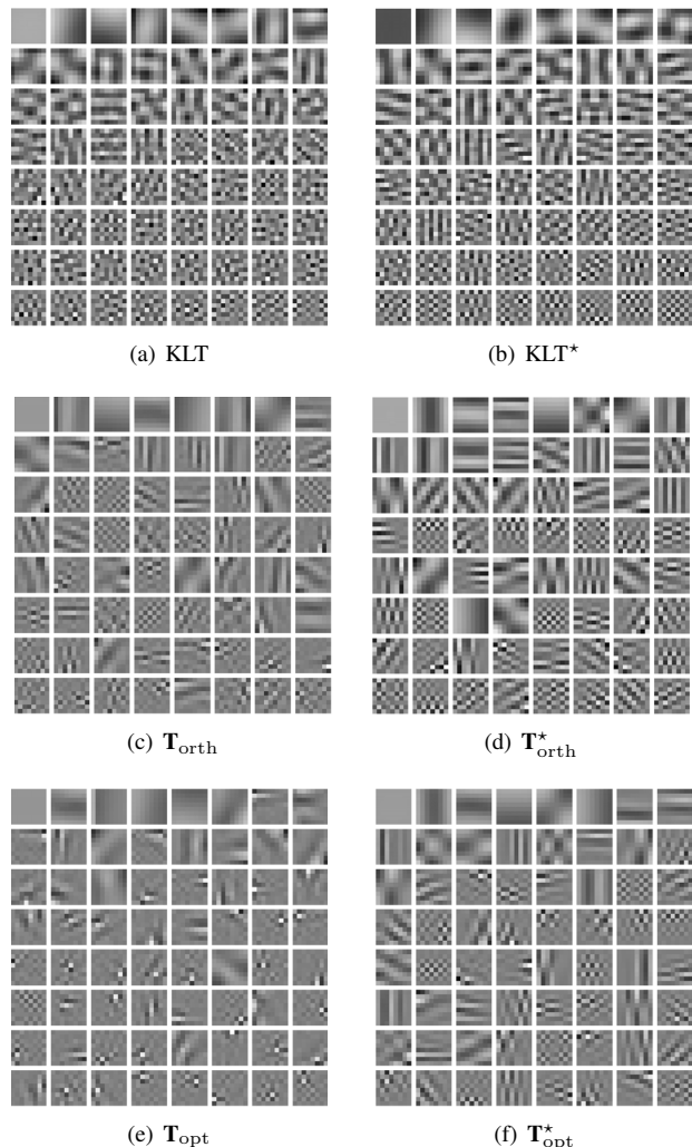
Fig. 1. KLT, \mathbf{T}_{\text{orth}} and \mathbf{T}_{\text{opt}} basis vectors obtained from Peppers (on first column) and \text{KLT}^* , \mathbf{T}_{\text{orth}}^* and \mathbf{T}_{\text{opt}}^* basis vectors obtained from the image training set (on second column).
