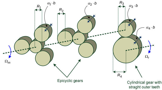
Figure 2: Speed reducer structure.
