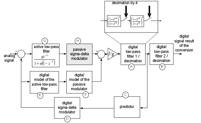
Figure 4. Active fast topology
