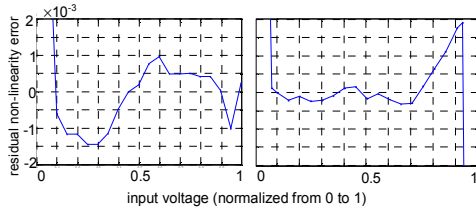
Figure 10. Non-linearity measurement
