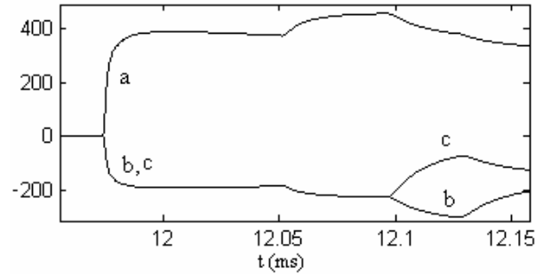
Fig. 3 After-fault residual current waves in a three feeder cable system 18.4+12.1+9.7\text{km} , a solid fault of R_f=1\Omega resulting in important amplitudes. \delta_{ip}=0.123\text{ms}
