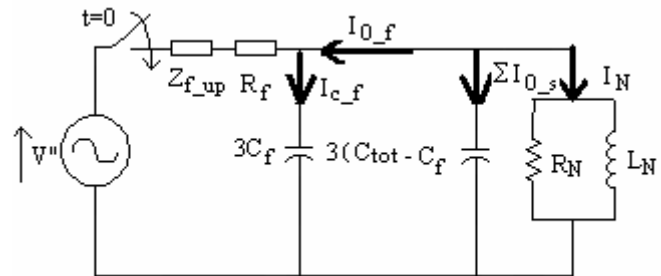
Fig. 7. An equivalent residual circuit of the faulty network on Fig. 3
