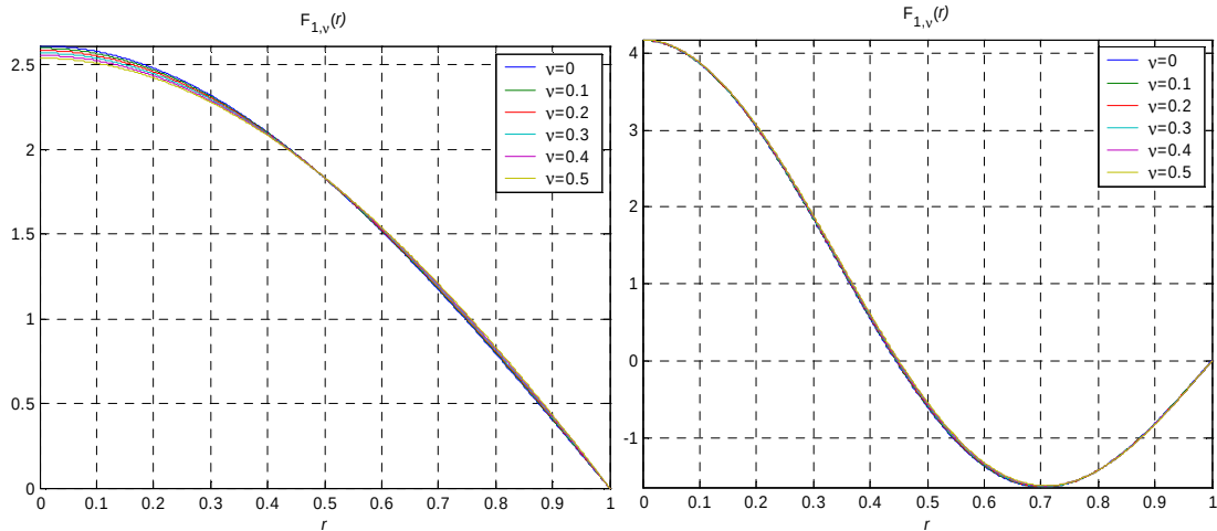
fig. 3: first two mode shapes of the Airy stress function for different values of Poisson's coefficient. Coefficients B_k have been chosen so that the mode shapes are orthonormal.
