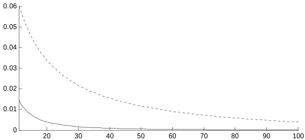
fig. 5: relative error as a function of number of quadrature points for the first integrals
