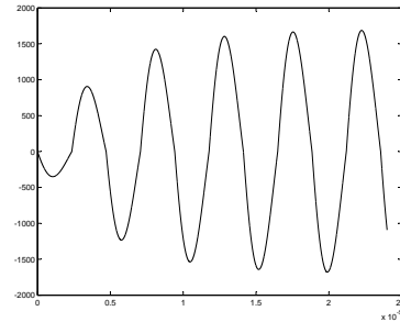
Fig. 2. Plate Velocity
