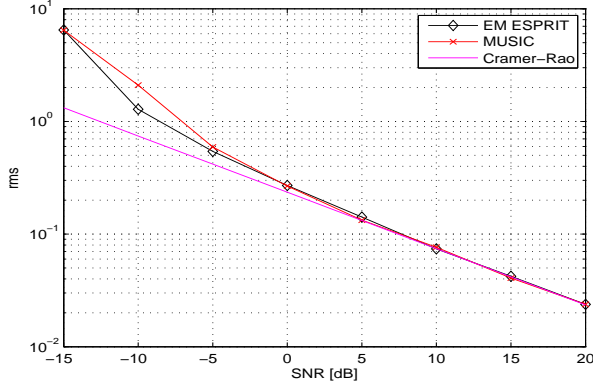
Fig. 3. RMS error for the source at -5^\circ for the array \mathbf{d} = [1, 2.32, 4.03, 6] \frac{\lambda}{2} , N = 2 sources.
