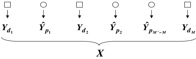
Fig. 1. Example of NLA and its equivalent VULA, with \mathbf{d} = [1, 3, 6] \frac{\lambda}{2} , \mathbf{p} = [2, 4, 5] \frac{\lambda}{2} and \ell = [1, 0, 1, 0, 0, 1] . □: existing sensors ( \mathbf{Y} ), ○: omitted sensors ( \hat{\mathbf{Y}}_{\mathbf{p}} ).
