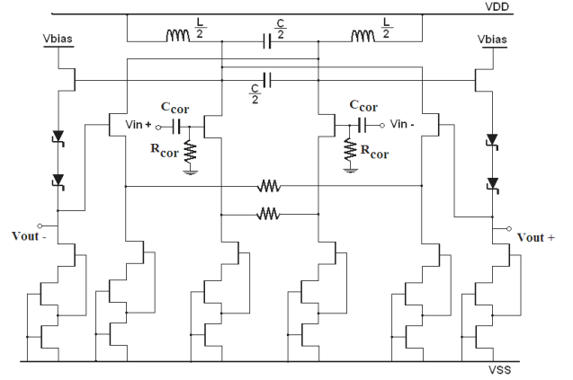
Figure 5: resonator circuit
