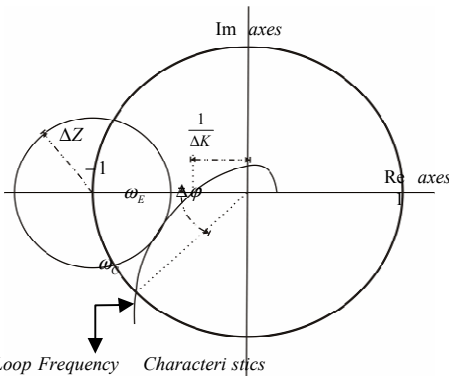
Fig. 2. Modulus ( \Delta z ), gain ( \Delta K ) and phase ( \Delta\phi ) margins for an open loop frequency characteristics
