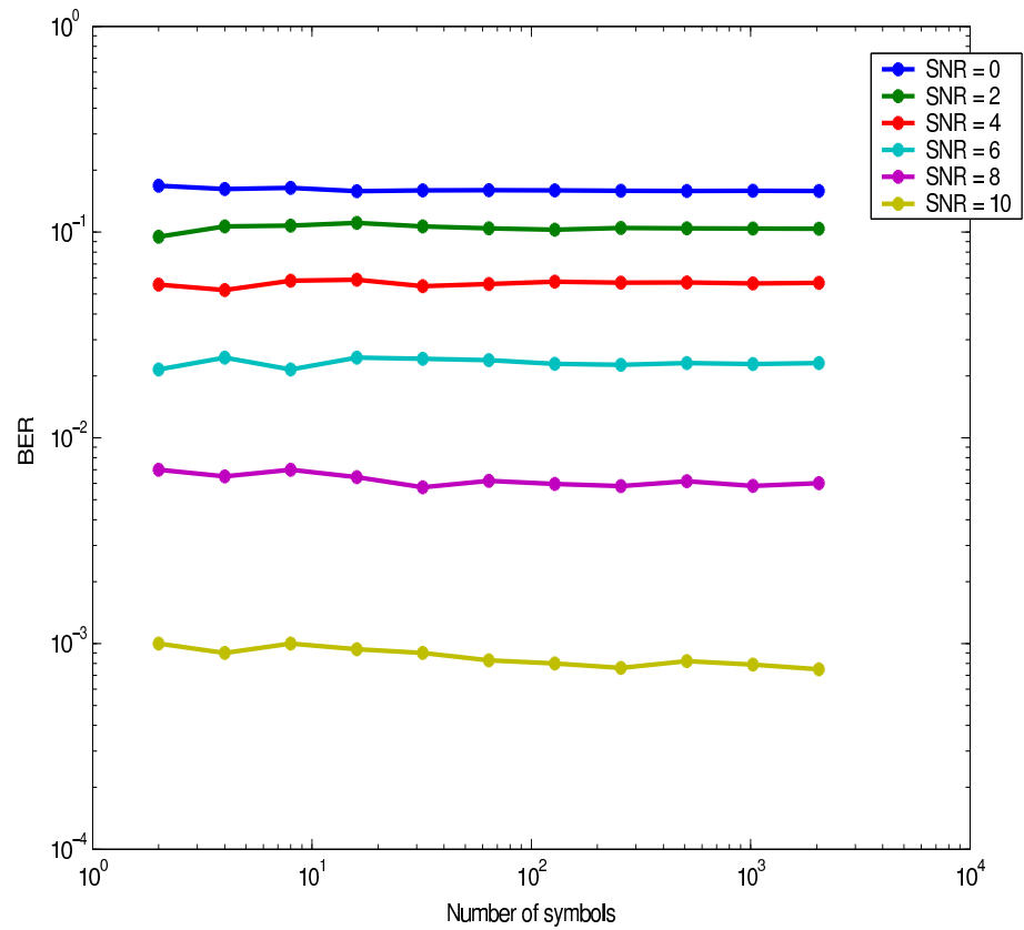
Fig. 3. BER v.s number of symbols ( M ) in dB for BPSK in AWGN using power detection where SNR are in dB.
