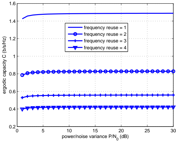
Fig. 7. The impact of the frequency reuse on the ergodic capacity, for frequency reuse of 1, 2, 3 and 4.
