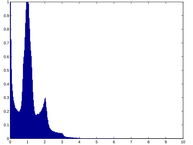
Fig. 6. Histogram of the mean eigenvalue distribution of 640 samples of \mathbf{V}^H \mathbf{V} , with \mathbf{V} a 1600 \times 800 Vandermonde matrix with uniformly distributed phases.
