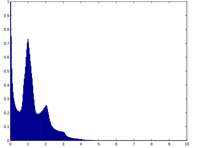
Fig. 5. Histogram of the mean eigenvalue distribution of 640 samples of \mathbf{V}^H \mathbf{V} , with \mathbf{V} a 1600 \times 1200 Vandermonde matrix with uniformly distributed phases.
