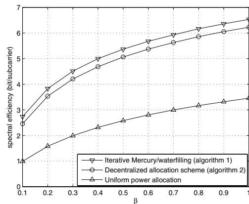
Fig. 3. Spectral efficiency comparison.
