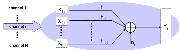
Fig. 1. N parallel Gaussian multiple access channels.
