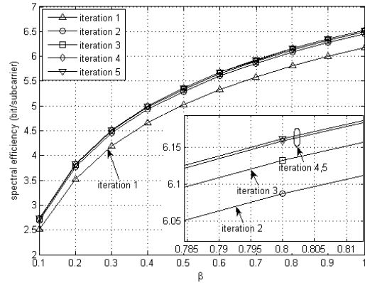
Fig. 2. Convergence of iterative Mercury/waterfilling.
