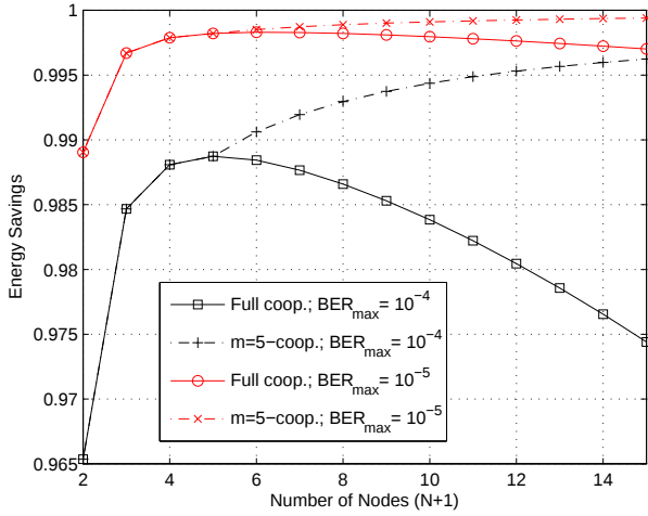
Fig. 2. The average energy savings curves versus the number of transmitting nodes, (N + 1) , employing full-cooperation and m -cooperation with two different \text{BER}_{\max} constraints.
