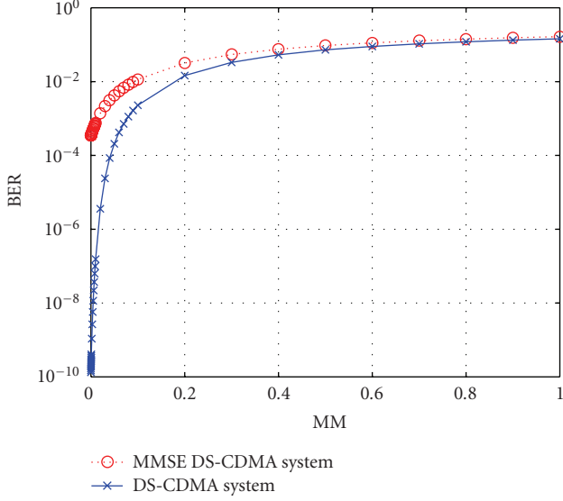
FIGURE 6: BER versus MM performances of the MMSE DS-CDMA system ( \cdots \circ \cdots ) and the proposed DS-CDMA system ( - \times - ), when l = 0 , M = 7 , L = 5 , N = 5 , and E_b/N_0 = 20 dB in all cases.
