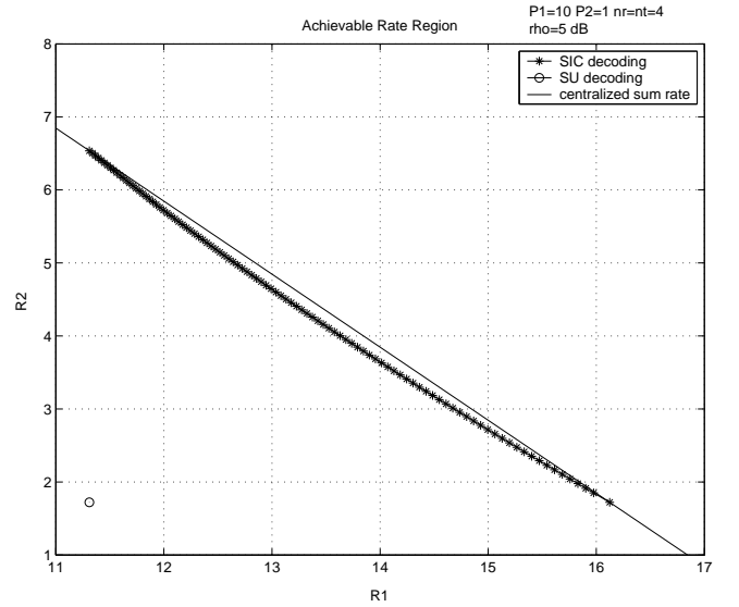
Fig. 2. Achievable rate pairs for the temporal power allocation case for P_1 = 10 , P_2 = 1 , n_r = n_t = 4 , \rho = 5 dB. The performance of the decentralized MAC with coordination is close to that of its centralized counterpart.
