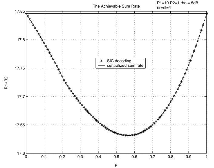
Fig. 1. Temporal power allocation case. MAC sum-rate versus p for P_1 = 10 , P_2 = 1 , n_r = n_t = 4 , \rho = 5 dB. The sum-rate of fading MIMO MACs is almost reached whatever the coordination signal distribution.
