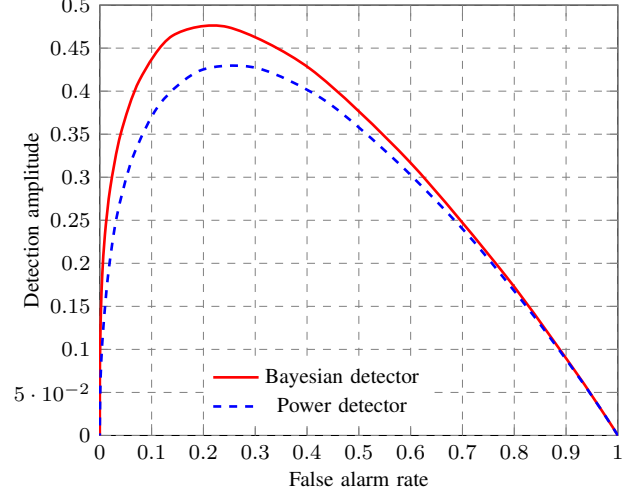
Fig. 1. Detection amplitude comparison in SIMO - M = 1 , N = 8 , L = 20 , \text{SNR} = -10 dB
