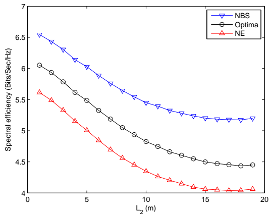
Fig. 4. System spectral efficiency vs. L_2
