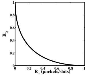
Fig. 3. Rate region of a collision channel with two users
