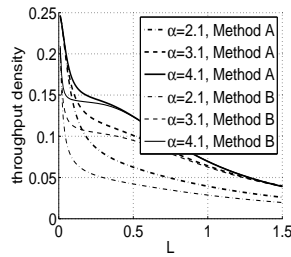
Fig. 12. Throughput density vs L for different \alpha and decoding schemes comparing MethodA with MethodB .
