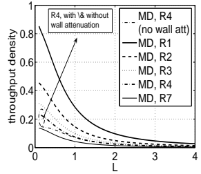
Fig. 14. Throughput density vs L for \alpha = 4.1 and different reuse factors (BS indoors).
