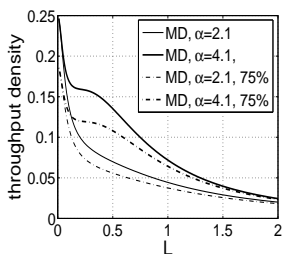
Fig. 18. Throughput density vs L for 100 % and 75 % cell coverage ( \alpha = 4.1 , multi-user detection, 2D).
