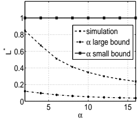
Fig. 9. Optimal cell size L^* vs path-loss factor \alpha (reuse factor m = 1 )
