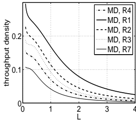
Fig. 13. Throughput density vs L for \alpha = 4.1 and different reuse factors.
