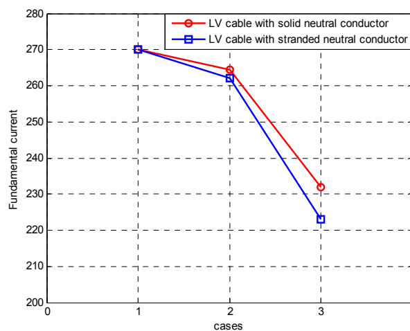
Fig. 8 Influence of harmonics on the transport capacity
