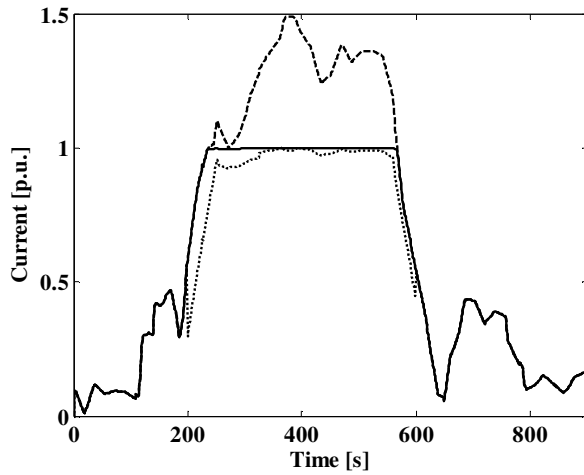
Figure 10: Evolution of the line current. 1 p.u represents the thermal current limit. Dash-dotted line: Without congestion management. Full line: With real-time supervisor. Dotted line: With actual method.
