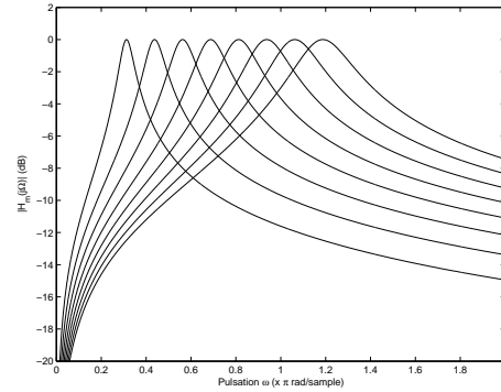
Fig. 6. Analysis filter bank magnitude responses
