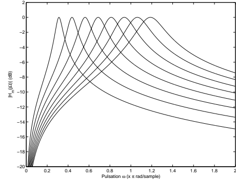
Fig. 6. Analysis filter bank magnitude responses
