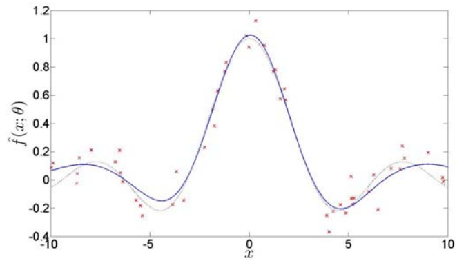
Fig. 2. Typical regression.
