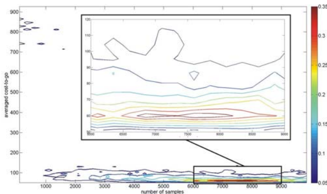
Fig. 9. Mountain car.
