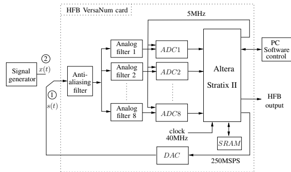
Fig. 7. Principle of HFB ADC calibration: channel adaptive equalization.
