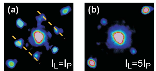
Figure 2: (a,b) Bandgap inhibition of instability modes for k_L \simeq \sqrt{3}k_P and two different lattice intensities. I_P > I_{TH} .
