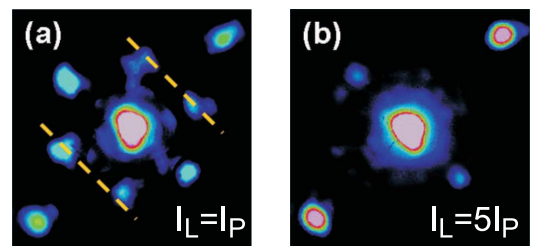
Figure 2: (a,b) Bandgap inhibition of instability modes for k_L = \sqrt{3}k_P and two different lattice intensities. I_P > I_{TH} .
