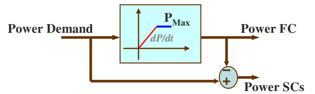
Fig. 3. Power Management Principle
