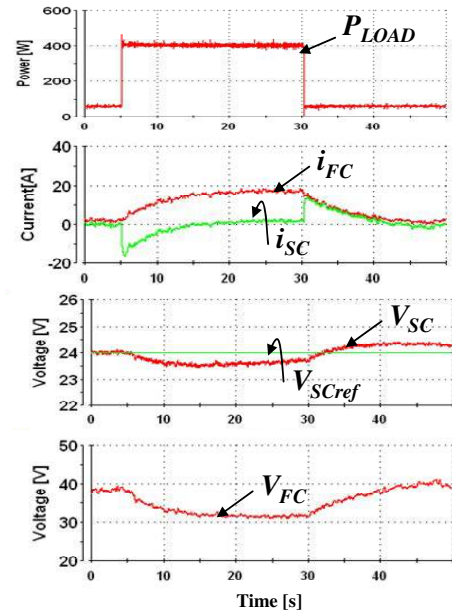
Fig. 7. Response of FC/ SCs system
