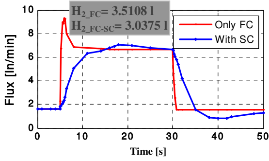
Fig. 8. Hydrogen mass flow consumption.
