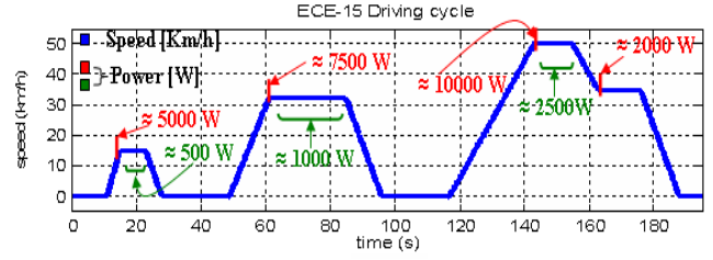
Fig. 2. ECE-15 driving cycle.
