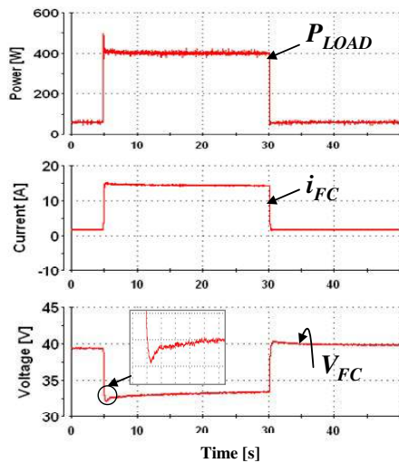
Fig. 6. Response of FC system
