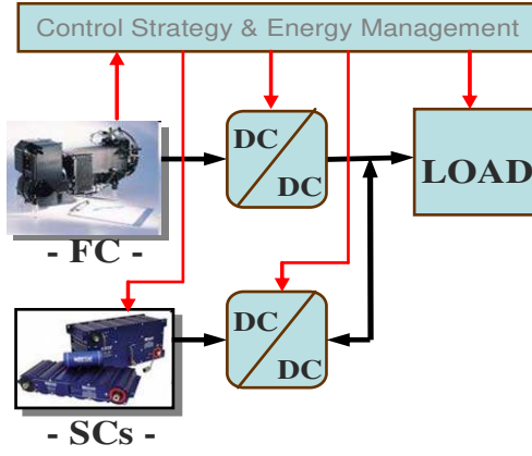
Fig. 1. Block diagram of a hybrid power system.
