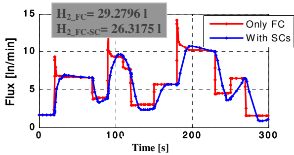
Fig. 10. Hydrogen mass flow consumption.
