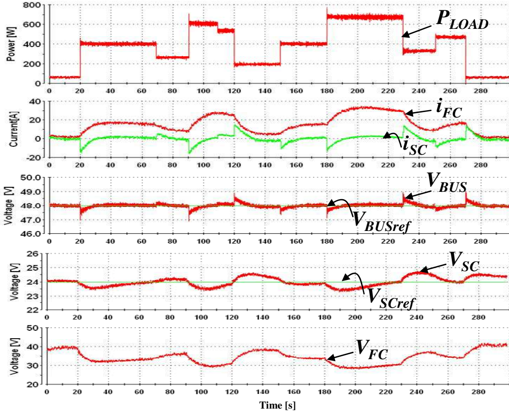
Fig. 9. Response of FC/SCs system for a complete load.
