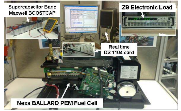
Fig. 5. Photograph of test bench.
