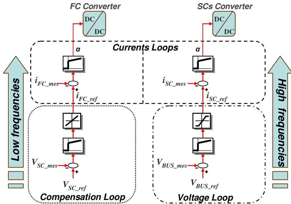
Fig. 4. Block diagram of control-command management strategy
