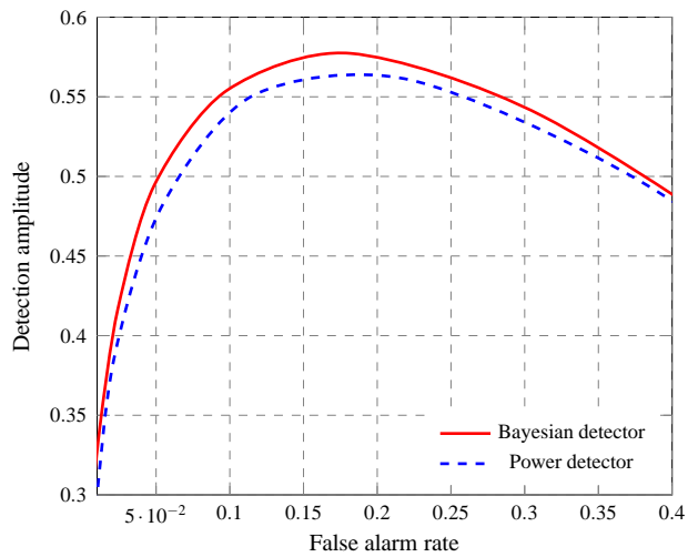
Fig. 2. Detection amplitude comparison in MIMO - M = 2 , N = 8 , L = 10 , \text{SNR} = -10 dB
