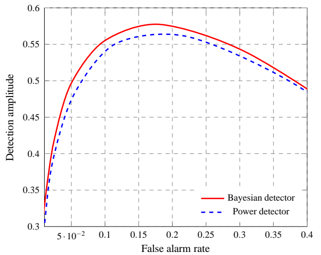
Fig. 2. Detection amplitude comparison in MIMO - M = 2 , N = 8 , L = 10 , \text{SNR} = -10 dB
