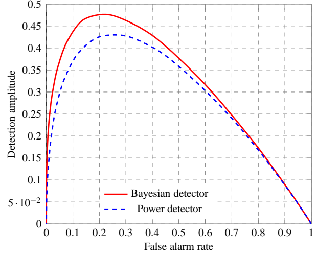
Fig. 1. Detection amplitude comparison in SIMO - M = 1 , N = 8 , L = 20 , \text{SNR} = -10 dB
