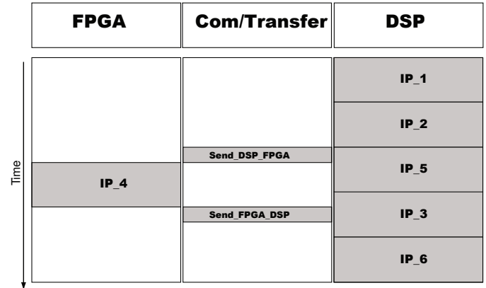
Fig. 11. Fully automatic scheduling obtained with one IP on the FPGA.
