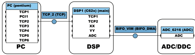
Fig. 15. SynDEX Pentek hardware platform graph.
