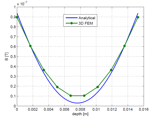
Fig. 10-b. Comparison between analytical and FE computation of magnetic flux density along the Oz axis of the magnet, at 8 kHz
