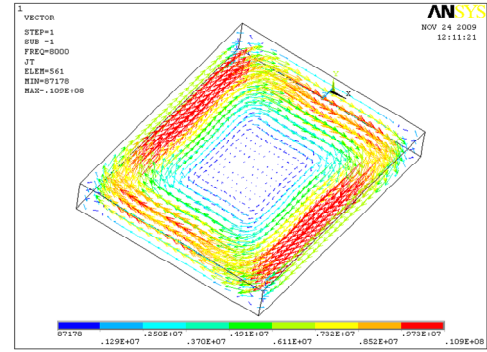
(b) Eddy-current with skin effect at frequency f=8\text{kHz}
