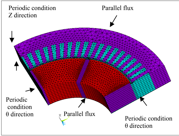
Fig. 1. Geometry of finite element model one pole-pair of the PM synchronous machine under study
