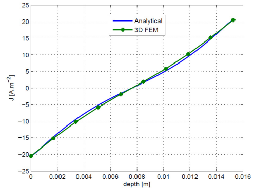
Fig.11-b. Comparison between analytical and FE computation of induced eddy-current densities along the Oz axis of the magnet, at 8 kHz
