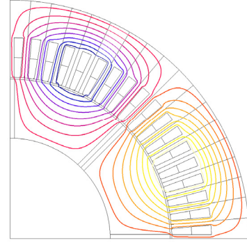
Fig. 2. Flux lines when stator current reaction is in line with q-axis.
