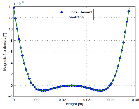
Fig. 9. Comparison between analytical and FE computation of induced eddy-currents along Ox axis in the magnet, at 8 kHz
