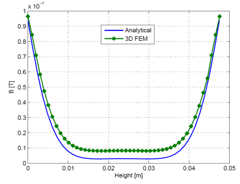
Fig. 10-a. Comparison between analytical and FE computation of magnetic flux density along the Ox axis of the magnet, at 8 kHz
