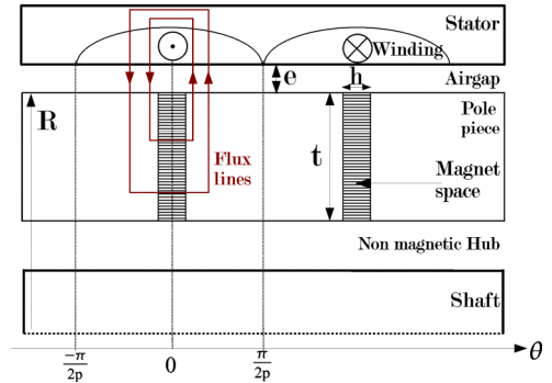
Fig. 4. Scheme for computation principle when stator current reaction phasor is in line with d-axis
