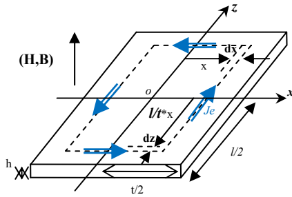
Fig. 5. Scheme of a magnet with eddy current paths
