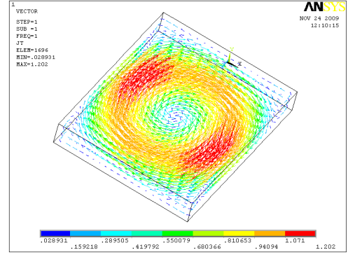
(a) Eddy-current without significant skin effect at f=1\text{Hz}
