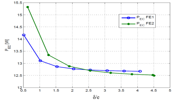
Fig. 7. Effect of mesh size on eddy-current losses in the magnet at harmonic frequency f=8\text{kHz} . The ratio of skin depth ( \delta=5.1\text{mm} ) versus element size ( e ) is varying along Ox and Oz .
