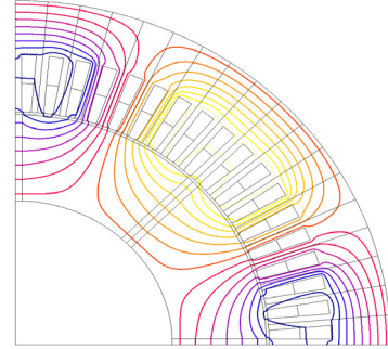
Fig. 3. Flux lines when stator current reaction is in line with d-axis.
