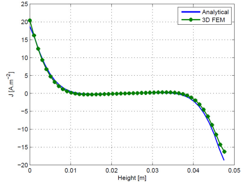
Fig. 11-a. Comparison between analytical and FE computation of induced eddy-current densities along the Ox axis of the magnet, at 8 kHz
