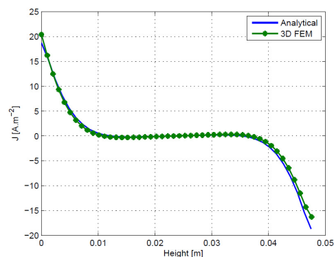
Fig. 11-a. Comparison between analytical and FE computation of induced eddy-current densities along the Ox axis of the magnet, at 8 kHz
