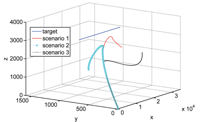
Fig. 3. Failed-interception trajectories
