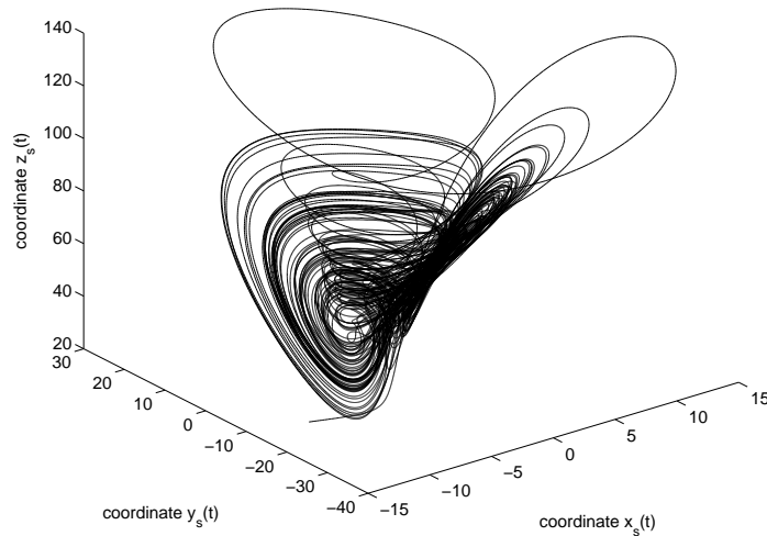
Fig. 2. Attractor of hyper-chaotic system without inputs i.e. , u_x = u_y = u_w = u_z = 0 – coordinates x - y - w
