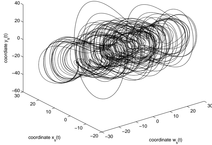
Fig. 3. Attractor of hyper-chaotic system without inputs i.e. , u_x = u_y = u_w = u_z = 0 – coordinates w - x - y
