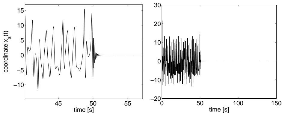
Fig. 4. Integral curve of coordinate x_s(t) , control action starts at t = 50s
