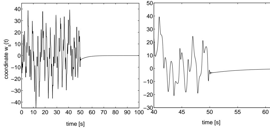
Fig. 7. Integral curve of coordinate w_s(t) , control action starts at t = 50 s
