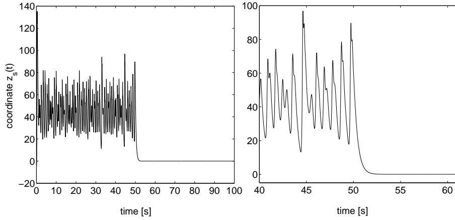
Fig. 6. Integral curve of coordinate z_s(t) , control action starts at t = 50 s
