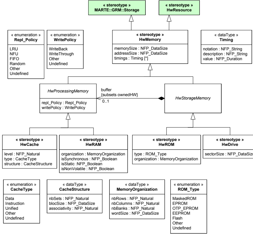
Fig. 2. HwMemory metamodel
