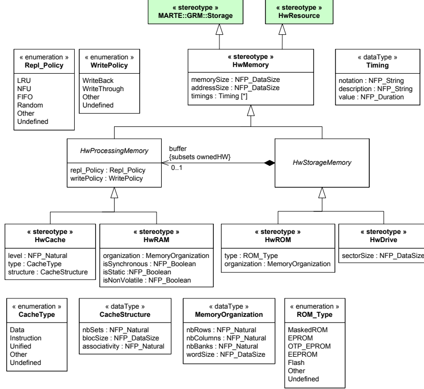
Fig. 2. HwMemory metamodel
