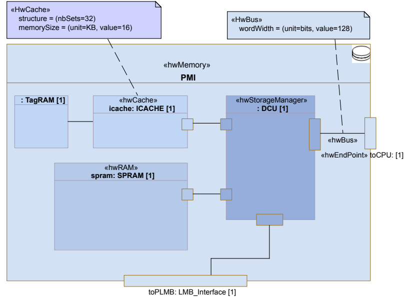
Fig. 4. PMI (Program Memory Interface) internal structure modeling
