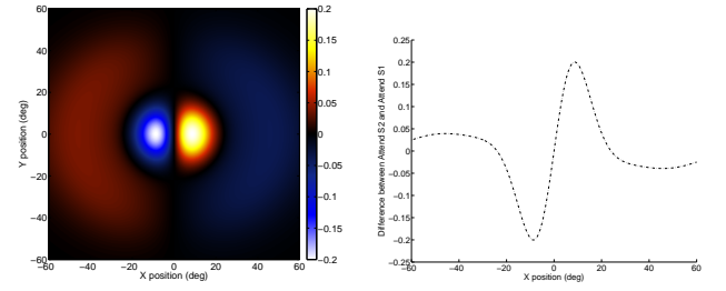
Figure 4: Illustrative example of the difference between the responses when attending S_1 ( x_{s1} = 15, y_{s1} = 0 ) and the responses when attending S_2 ( x_{s2} = -15, y_{s2} = 0 ) showing that a divisive model can qualitatively account for the difference maps observed in [3]. In order to produce this pattern, an influence between the probe and the anti-preferred stimuli has been introduced leading to a suppression by the anti-preferred stimuli that is stronger when a probe is flashed close to them. The illustration on the right is a slice of the difference map along the x-axis connecting S_1 , S_2 and the receptive field centre.
