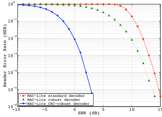
Fig. 9. Header Error Rate (HER) vs. SNR for the standard, robust, and CRC-robust decoders of the MAC-Lite layer.
