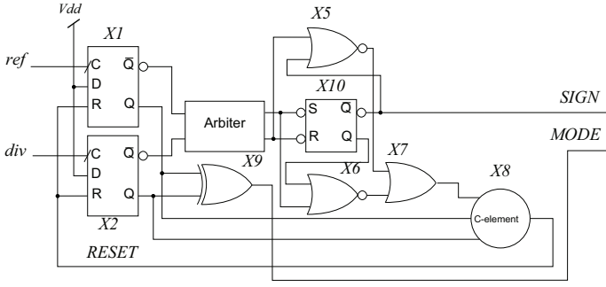
Fig. 5. Schematic of the bang-bang phase-frequency detector.
