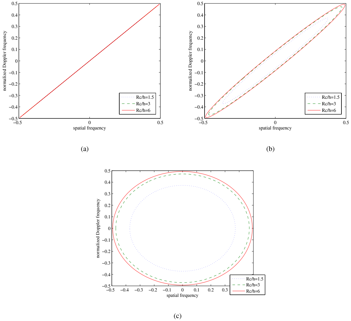
Fig. 2. Examples of the locus of clutter ridges in case of an ULA in monostatic configuration. (a) crab angle of \phi_a = 0^\circ ; (b) crab angle of \phi_a = 10^\circ ; (c) crab angle of \phi_a = 90^\circ
