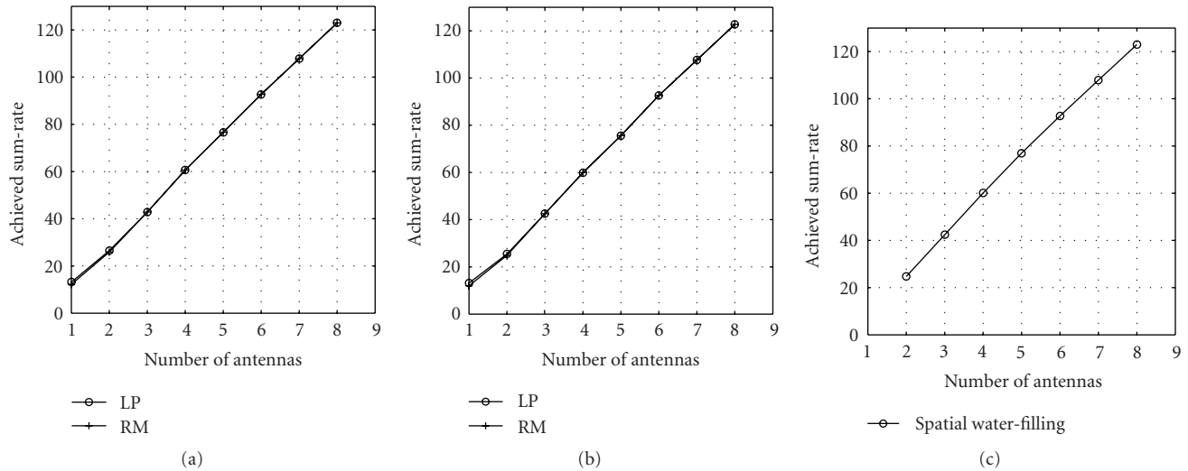
FIGURE 15: Achieved sum-rate versus the number of antennas for selected scenarios: (a) TSD-MIMO, (b) SVD-MIMO, and (c) spatial waterfilling reference line (LP: Linear Programming, RM: Regret Matching).
