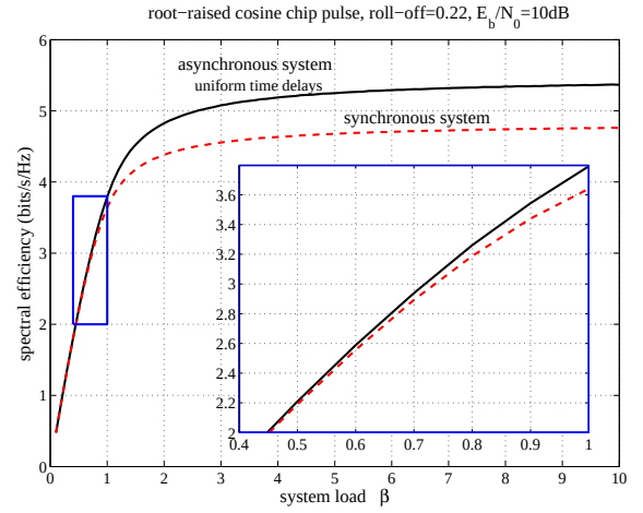
Fig. 2. Spectral efficiency of random CDMA versus the load \beta for the root-raised cosine chip pulse used in the UMTS standard and \frac{E_b}{N_0} = 10 dB.
