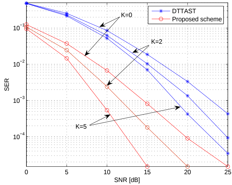
Fig. 4. Comparison of DTTAST codes and the proposed scheme with two unsynchronized relays over Rayleigh and Rician channels K \in \{0, 2, 5\} .
