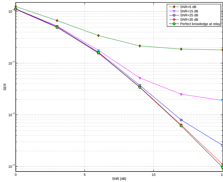
Fig. 5. Effect of wrong relaying on the performance of the proposed scheme with three unsynchronized relays over Rician channels K = 1 .
