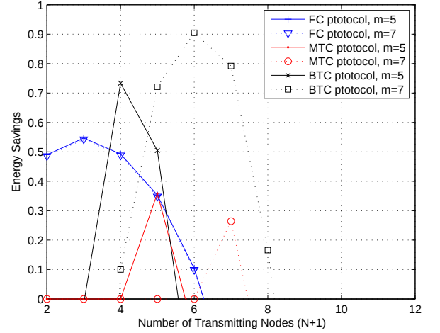
Fig. 2. The average energy savings curves versus the number of relays, using the distributed power allocation for cooperative routing with distributed space-time codes of m cooperating nodes when per hop outage probability requirement is \rho_0 = 10^{-5} .
